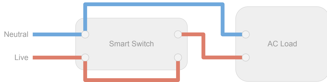
AC load wiring diagram, switching on live :
