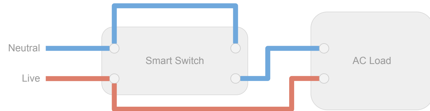
AC load wiring diagram, switching on neutral :
